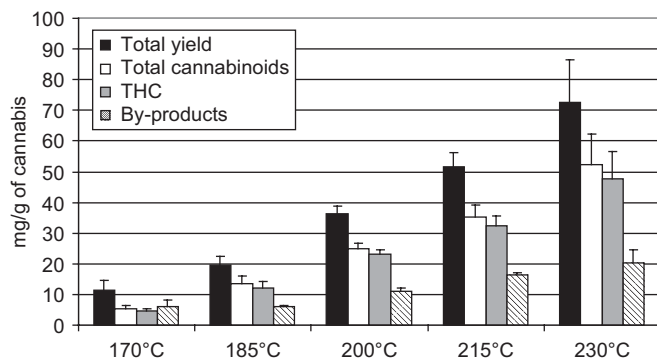
Figure 3. Analysis conducted on the Vaporiser in order to establish the differences in total yield, total cannabinoids, THC, and total by-products obtained when the samples are produced at five different temperatures.
