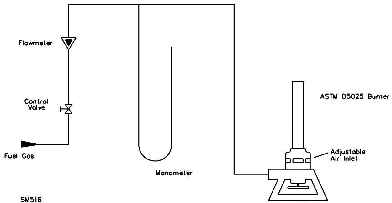
Figure 52.1 Burner supply arrangement
