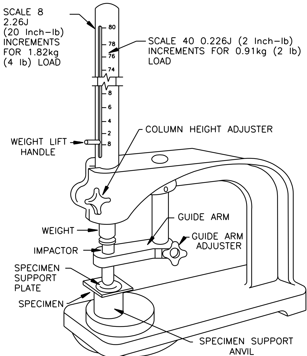
Figure 58.1 Impact tester
