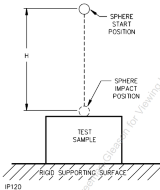
Figure 39.2 Ball drop impact test
