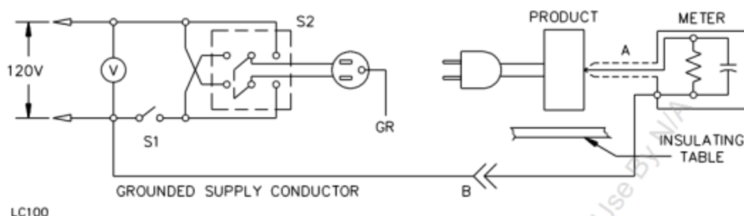
Figure 31.1 Leakage-current measurement circuit
