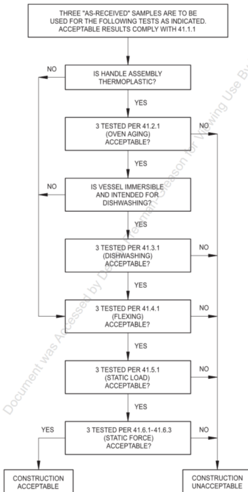
Figure 41.4 Handle strength test procedure
