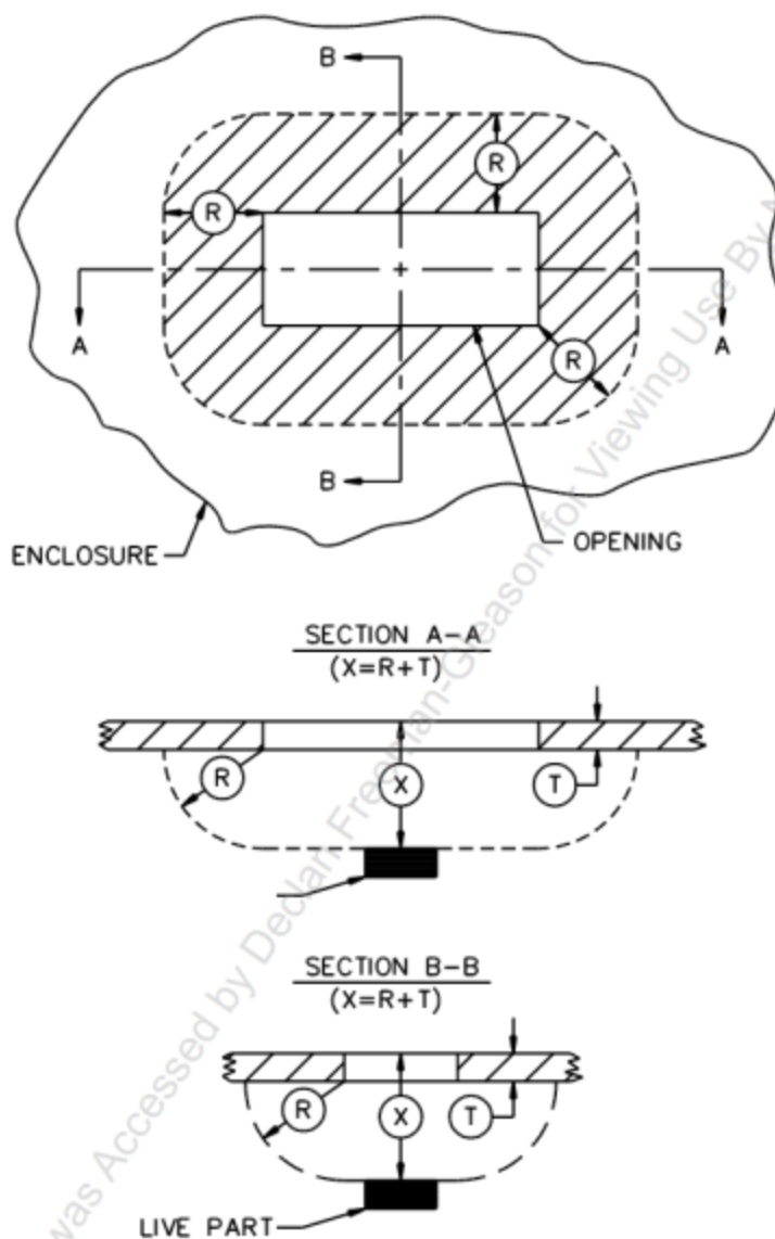
Figure 7.3 Opening in enclosure
