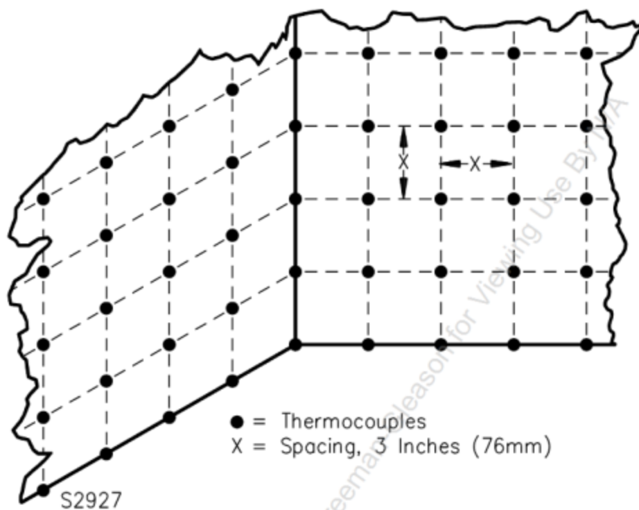
Figure 33.3 Thermocouple spacings
