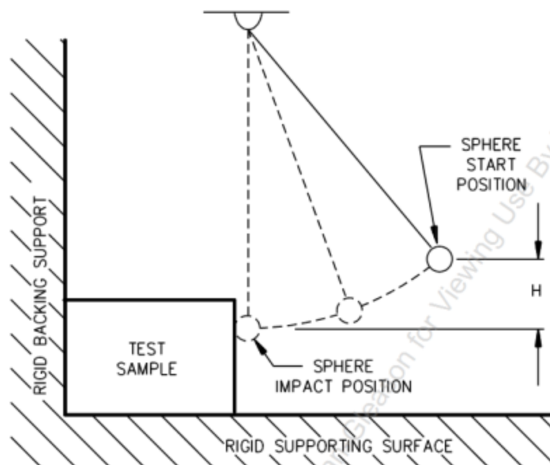
Figure 39.3 Ball pendulum impact test
