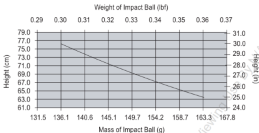
Figure 46.3 Pendulum Drop Height (H)
